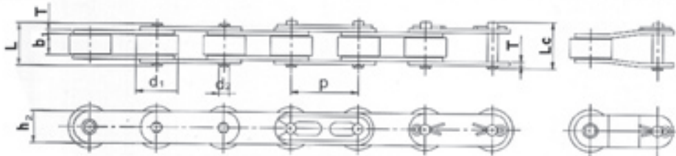
Large Roller Type
