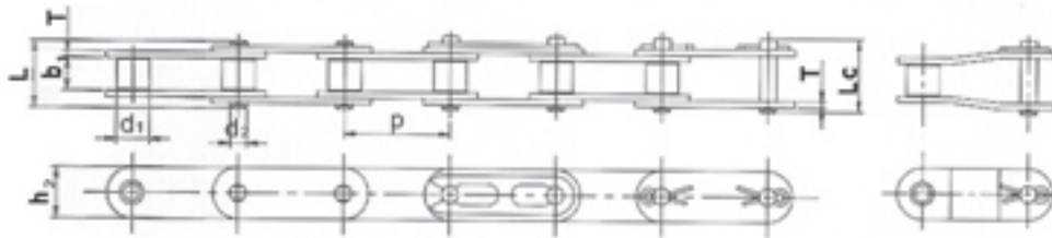
Small Roller Type
